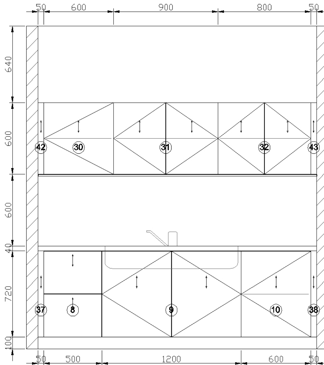
E View elevation drawing
