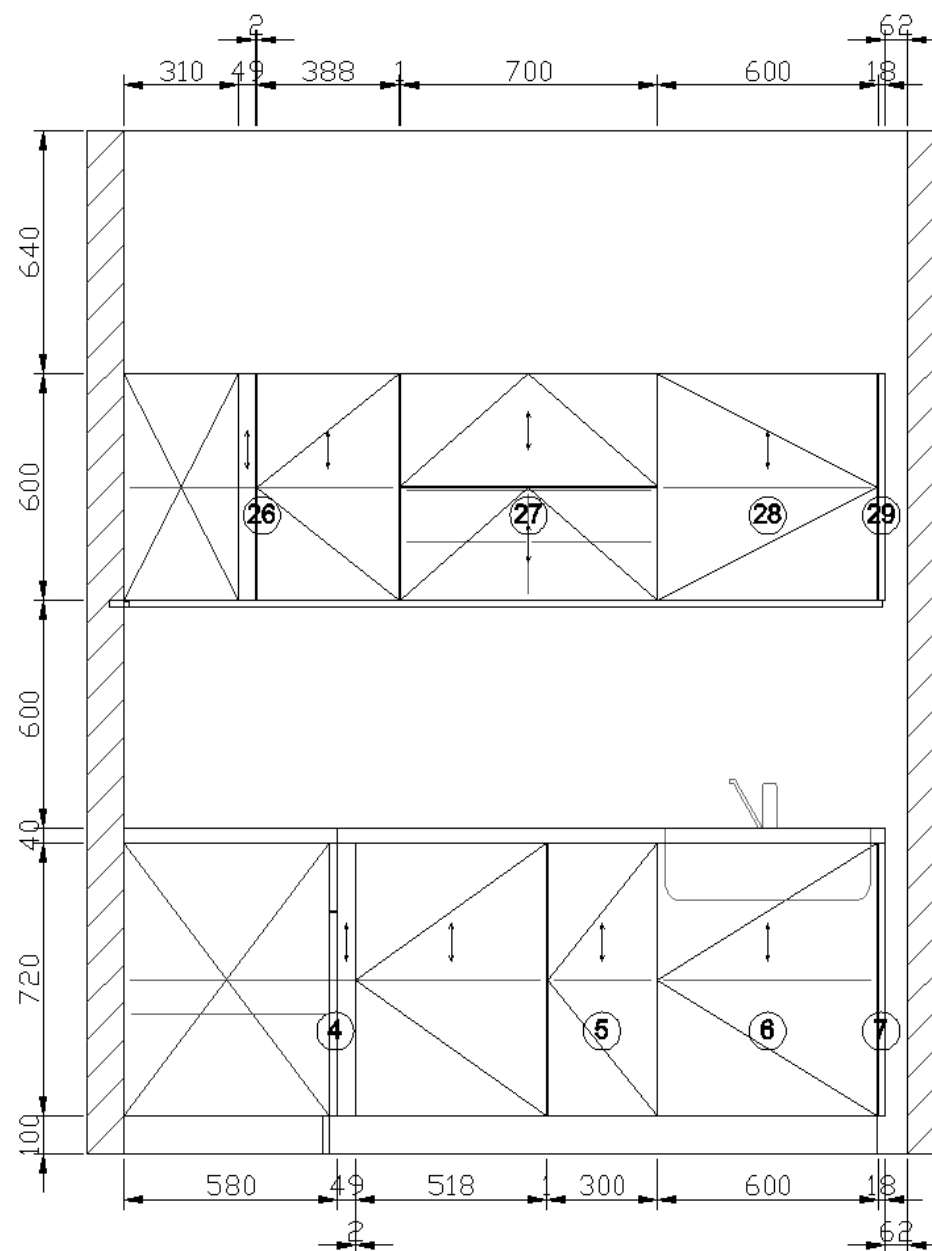
D View elevation drawing
