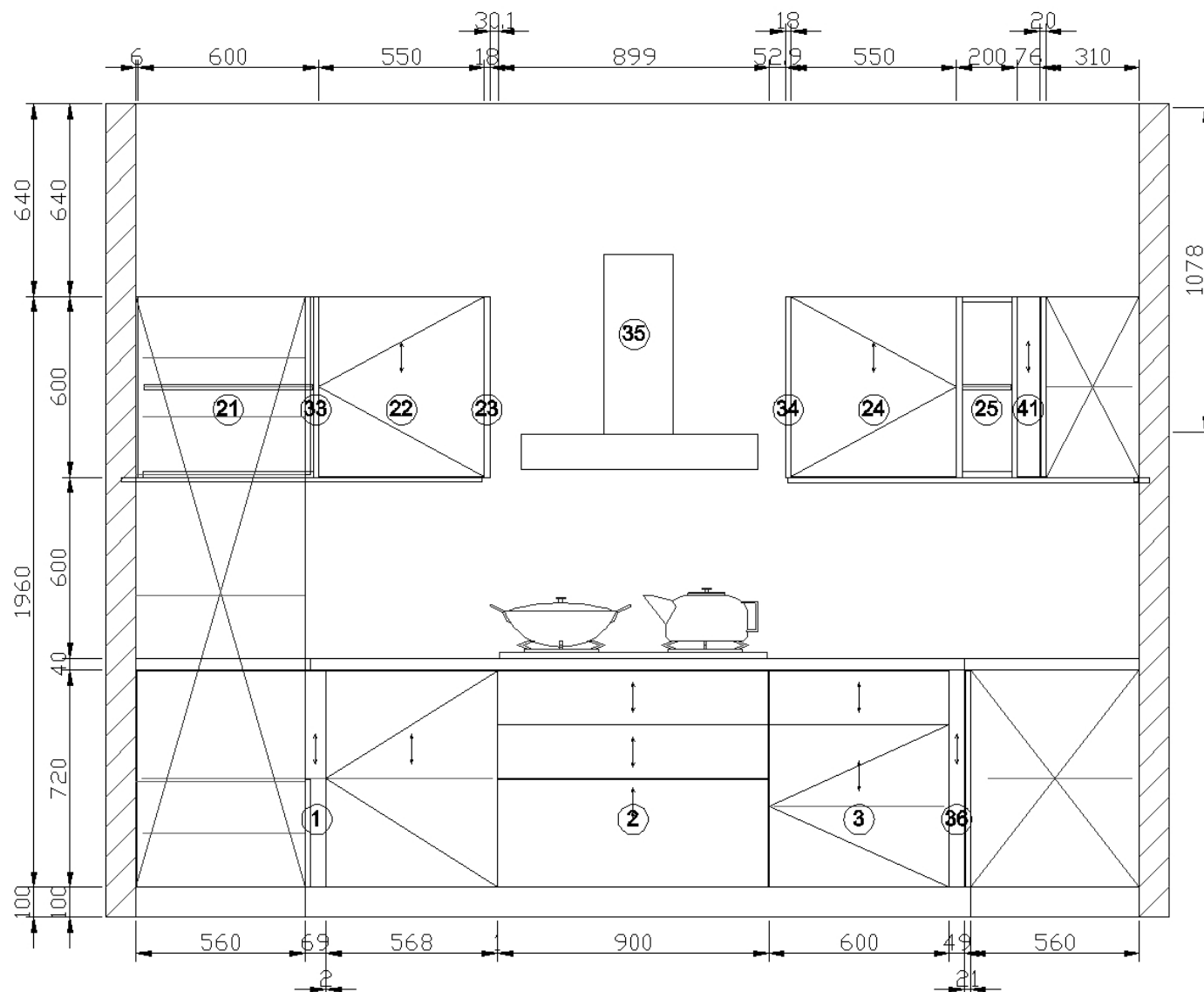
C View elevation drawing
